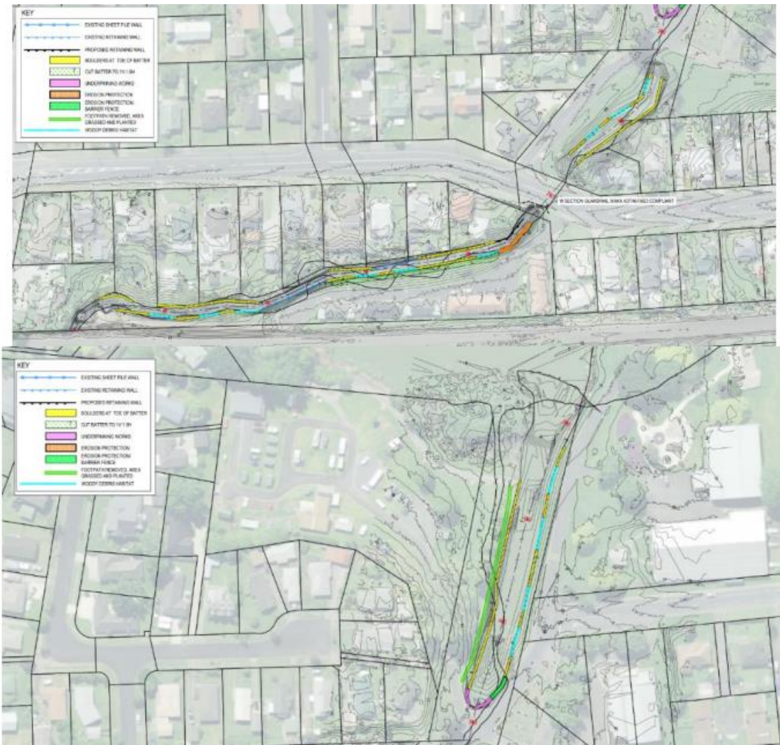
Hakanoa Stream Rehabilitation plans
