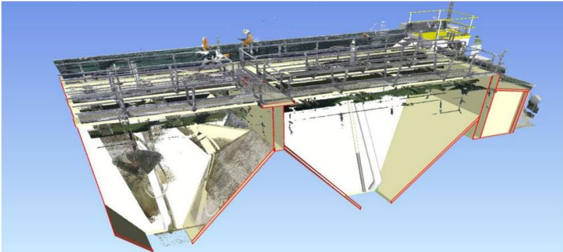
Ngaaruawaahia Water Treatment Plan Upgrade- Clarifier 3D point cloud detailing dosing and flow improvements
