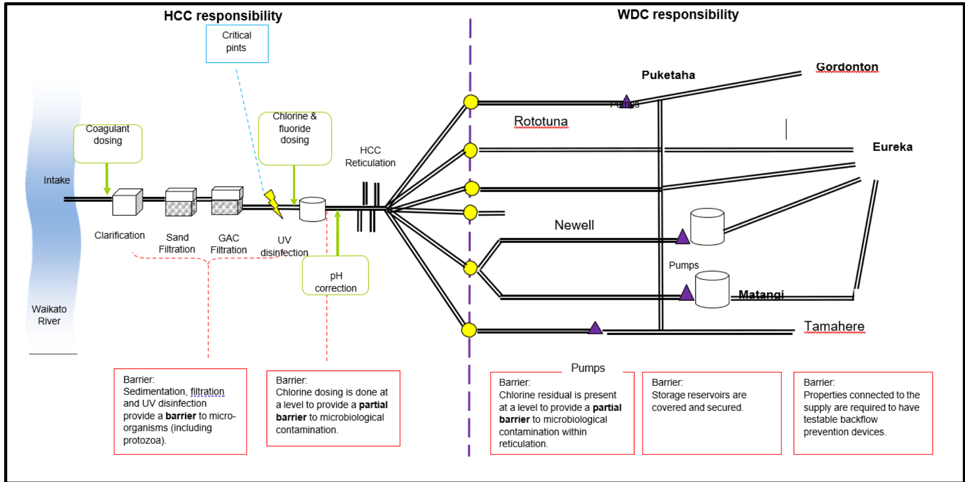
Figure 4: Water Supply Flow Diagram
